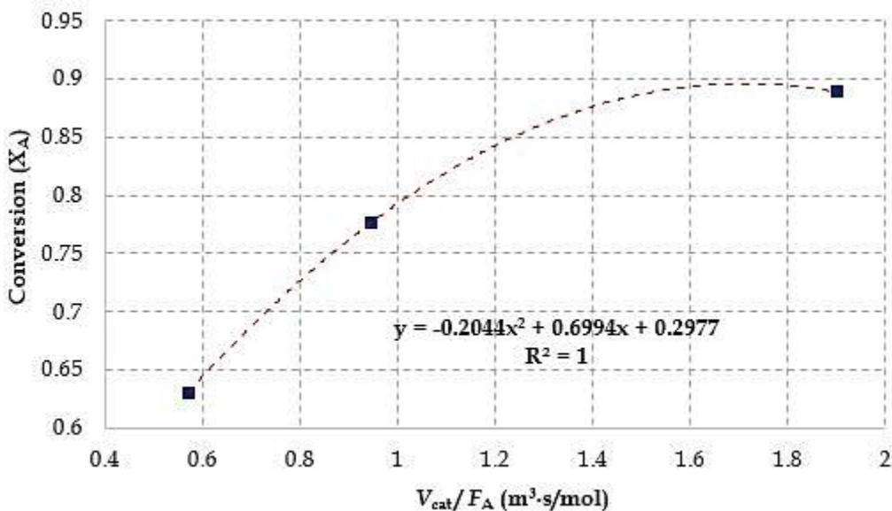
Figure 6. Ethanol Conversion ( X_A ) versus Reactants Space-Time ( V_{\text{cat}}/F_A )
