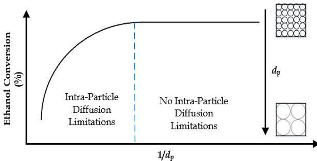
Figure 2. Experimental assessment of intra-particle diffusion limitation
