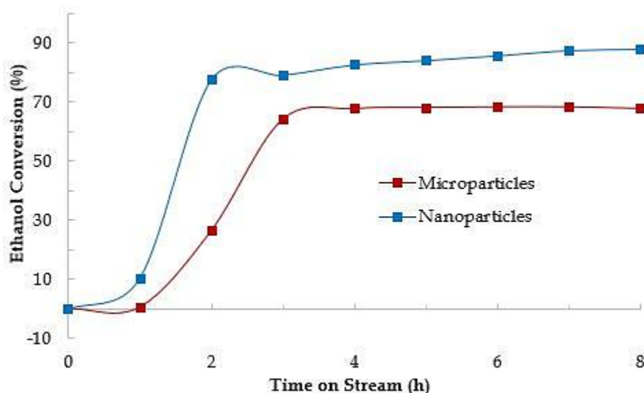
Figure 9. Ethanol conversion over time for micro and nanoparticles
