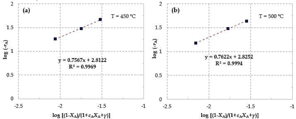
Figure 7. Log (-r_A) versus \log [(1-X_A)/(1+\epsilon_A X_A + \gamma)] for two evaluated temperatures: (a) 450 °C and (b) 500 °C.
