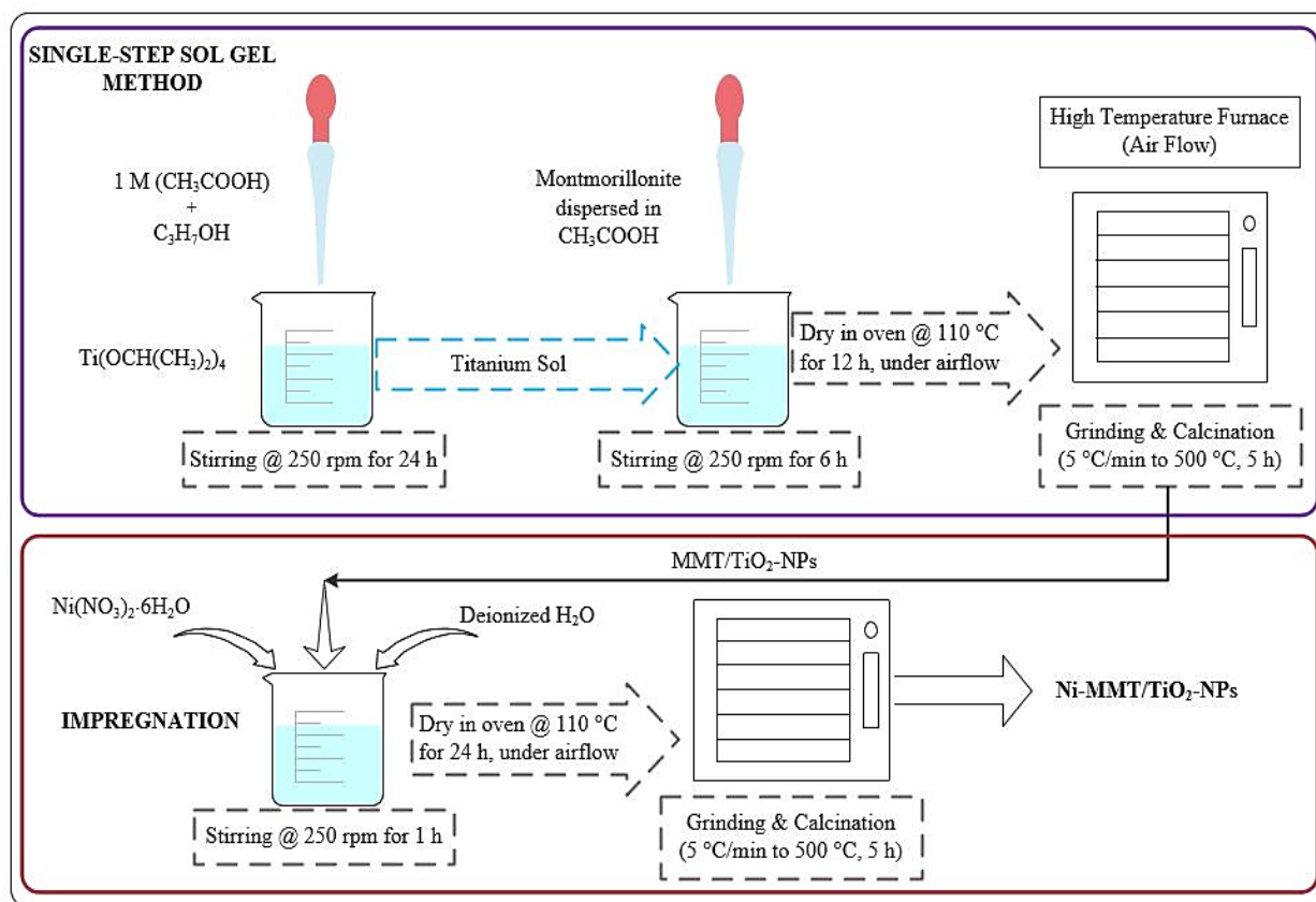
Figure 1. Catalyst synthesis process
