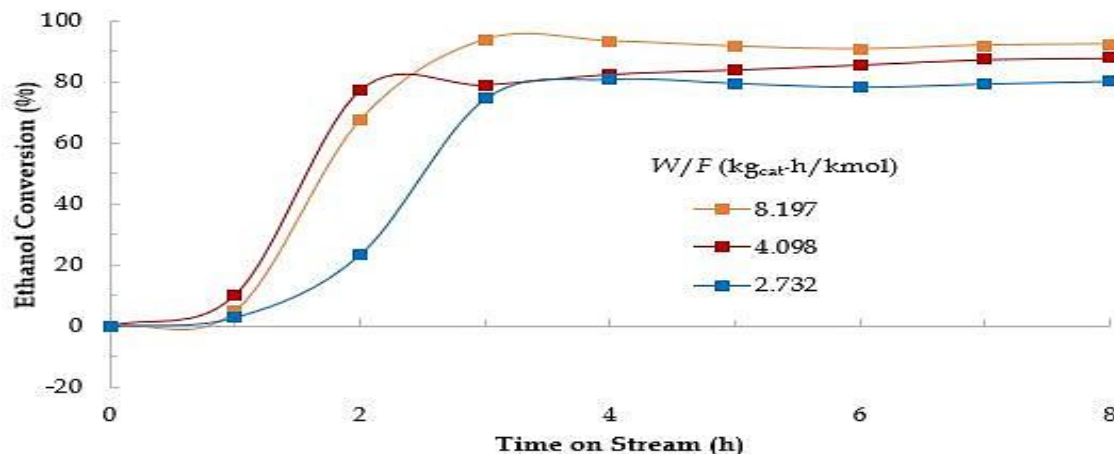
Figure 10. Conversion of ethanol and the effect of space-time on nanoparticle catalyst
